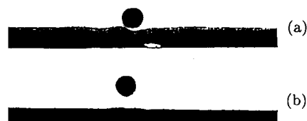
(a) e/D = 0 , Kc = 3.91 , Re = 1.25 \times 10^3 , \theta = 0.61 \times 10^{-4} , D = 28.9 mm (b) e/D = 0.73 , Kc = 8.22 , Re = 1.14 \times 10^3 , \theta = 0.89 \times 10^{-4} , D = 19.19 mm
